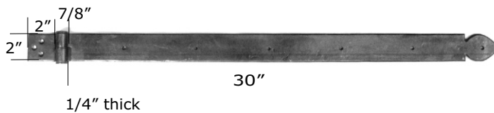
HB372 Pintle Strap Hinge. MUST SPECIFY HANDING (see handing chart on next page).
