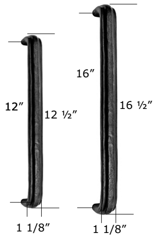
HP791AP-12 HP791AP-16 Monte Vista Pulls (2.25" projection)
