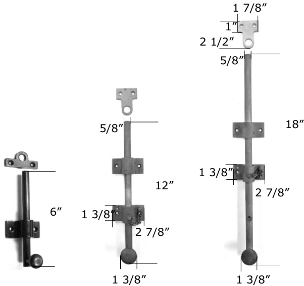
Knob Grip Surface Bolts
