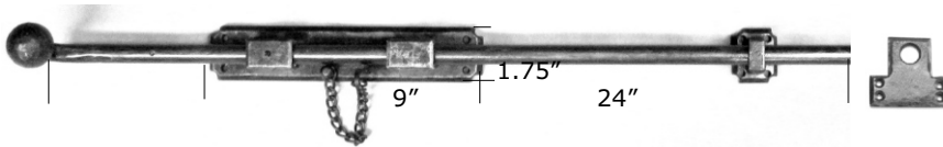
HB286 24" Dunn Surface Bolt
