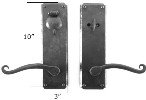
HE601 (shown w/ HL113 Lever)
