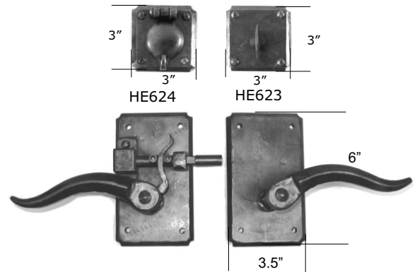
HS508 Santa Barbara Latch Entry (shown w/HL101)
