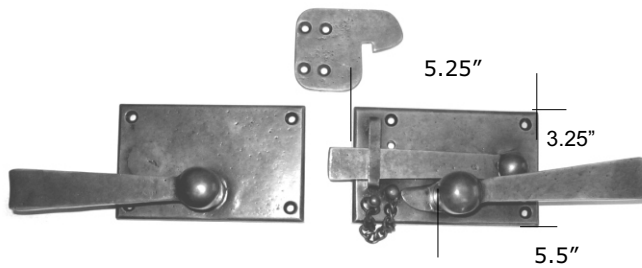
BS507 Bermuda Gate Latch (Privacy shown with locking chain. Emergency egress included). NO LEVER OPTIONS
