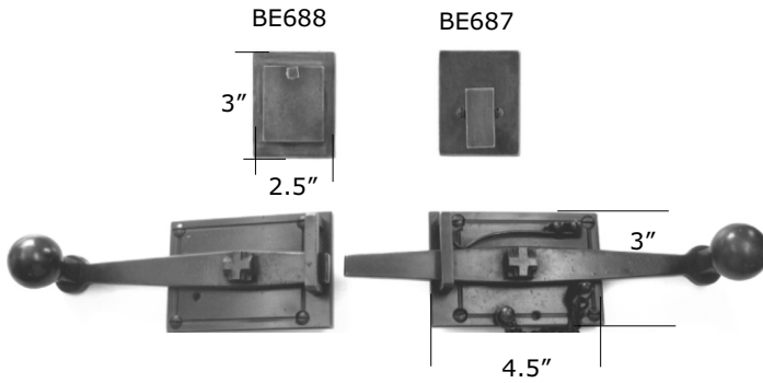
BS504 EN-DB Tweezer Strike-bar Latch with Tubular Deadbolt
