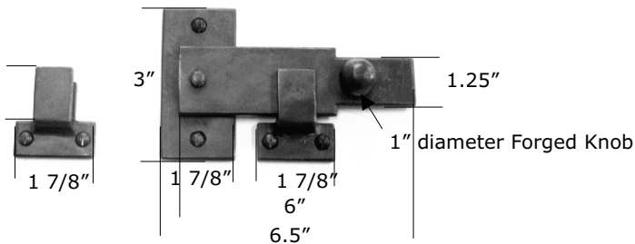
HS522 Barn Door Latch (ONE SIDE ONLY)
