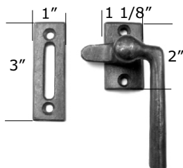
HW115 Casement Latch MUST SPECIFY HANDING (showing RH)
