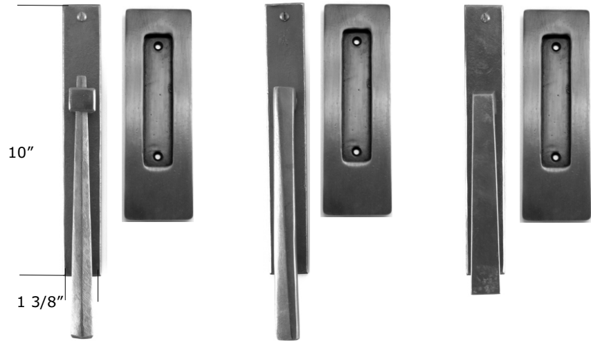
BE671 Escutcheon set shown w/ BL108L East-West 9" Lever & BP712 Flush Pull
