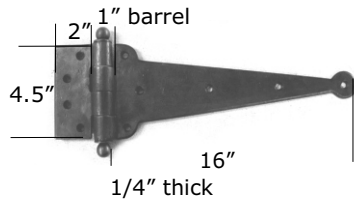
HB361 Full Barrel Heavy Duty Strap Hinge
