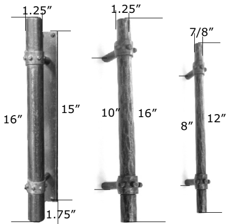
HP709-ESC HP709 HP709-12 Galisteo Pulls (3.5" projection)
