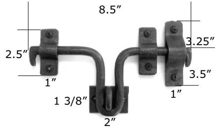
HB520 Slide Bolt 1 5/8" total projection
