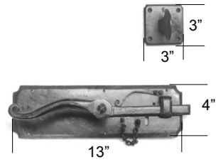
HS501 (shown w/HL113)
