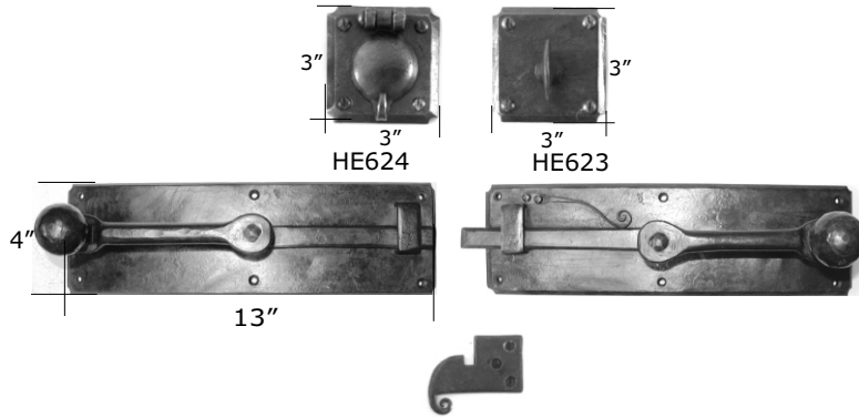
HS501 Horizontal Strike-bar Latch Entry (shown w/HL111 Lever)
