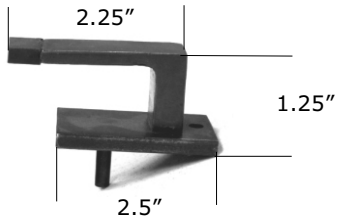
BD258 Contemporary Floor Stop
