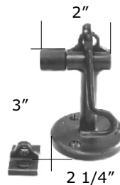
BD262W Floor Stop with Hook
