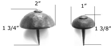
HC362 1" Dome HC363 2" Dome
