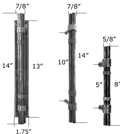
HP706-ESC HP706 HP706S Trio Pulls (3.5" projection)
