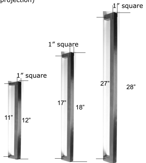
HP726AP-12 HP726AP-18 HP726AP-28 Stockholm Pulls (2.5" projection)
