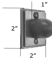
BD259 Wall Stop
