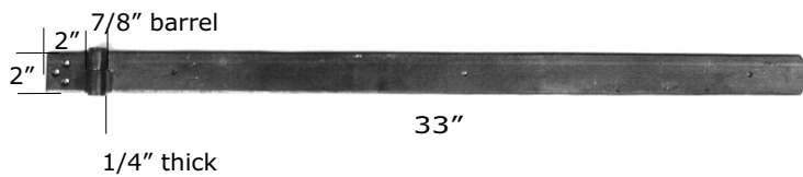
HB371 Pintle Strap Hinge. MUST SPECIFY HANDING (see handing chart on next page).
