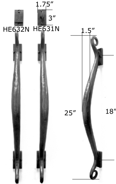
HP113 Scrolled Pull (4" projection)
