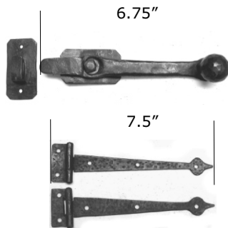
HG233 Latch & 2 Strap hinges
