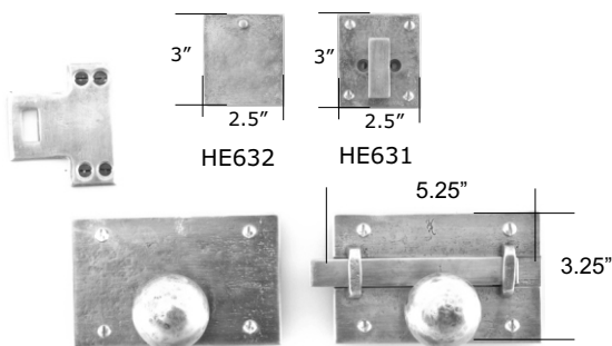
HS509 Scottsdale Latch Entry (No lever option)
