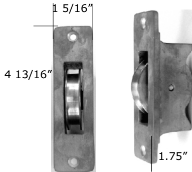
BW210 Window SASH PULLEY (with #25 natural bronze chain)
