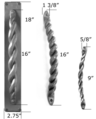
HP702-ESC HP702 HP703 Rope Pulls (4" projection)
