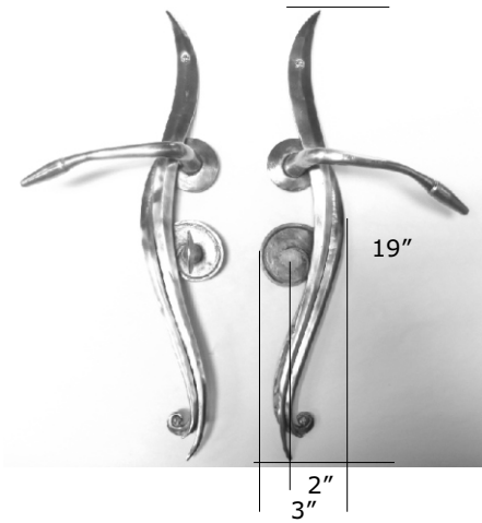
HL106MP Louvre (PATIO FUNCTION ONLY)
