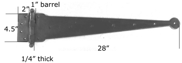
HB363 Full Barrel Heavy Duty Strap Hinge
