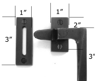
BW116 Milan Window CASEMENT LATCH (RH shown - SPECIFY HANDING!)
