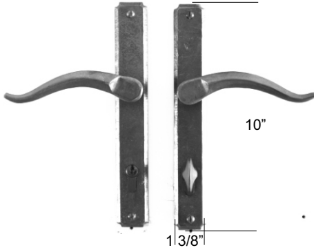
HE605 Straight Edge HE605B Beveled (square corners) HE605NC Notched Corner (shown) No spring assist (5" and smaller levers recommended)
