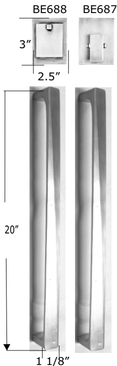
BP725L-20 Milan (2" projection)
