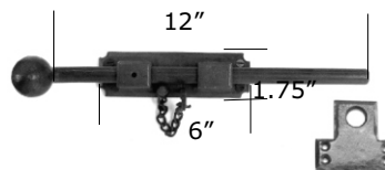
HB288 12" Dunn Bolt
