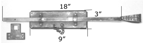
HB281 18" Surface Bolt
