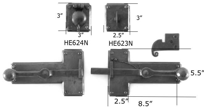
HS502 T-shaped Strike-bar Latch Entry (shown w/HL111)
