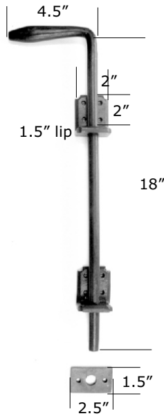
HB233 Cane Bolt
