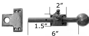
HB271 6" Narrow Guide Bolt 2.75" throw
