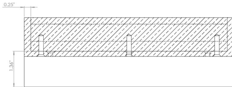
SECTION F-F
