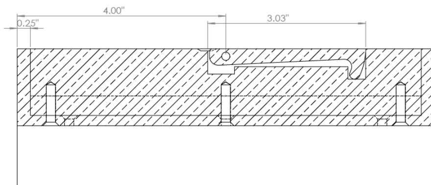
SECTION E-E
