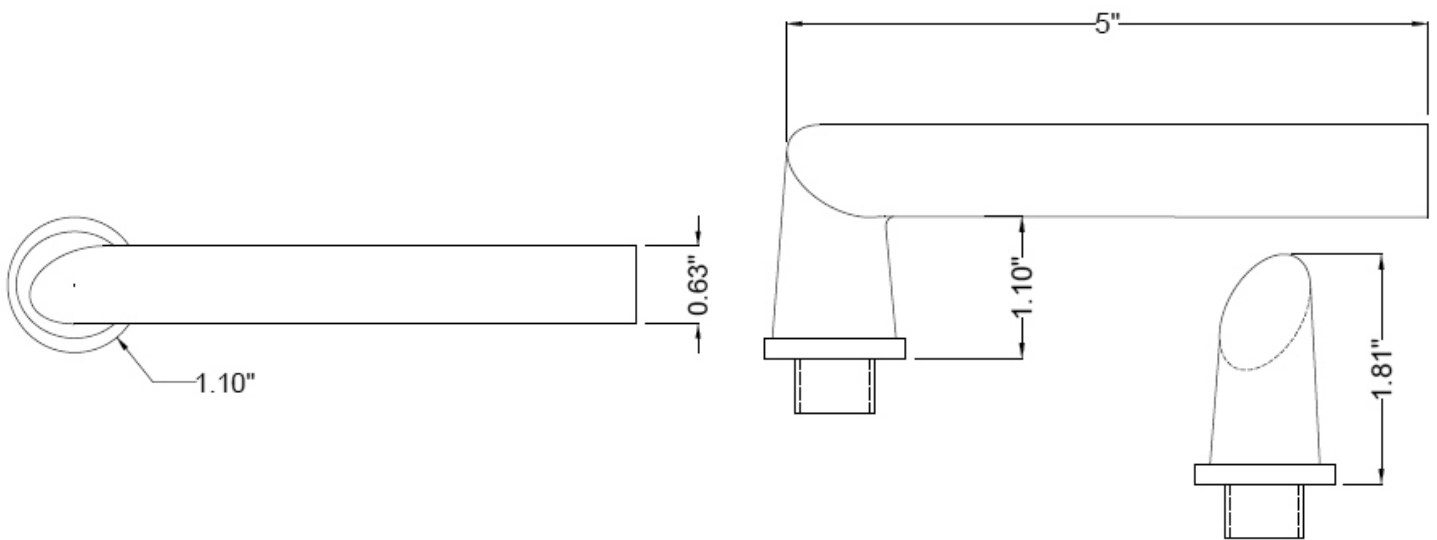
L180 Brass Turner Lever
